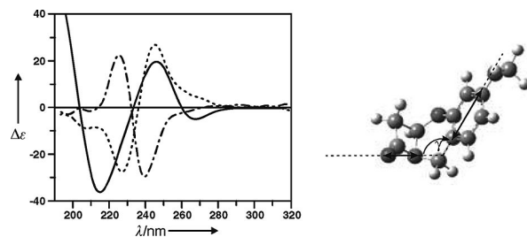
Figure 1. Experimental CD spectra of ent- 4a (---) and 4b (···) and simulated CD spectrum of 4b (—) (left). Lowest energy conformer of 4b calculated at the B3LYP 6-31G++ (d,p) level.
