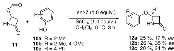
Scheme 4. Intermolecular enantioselective formation of 12 .
