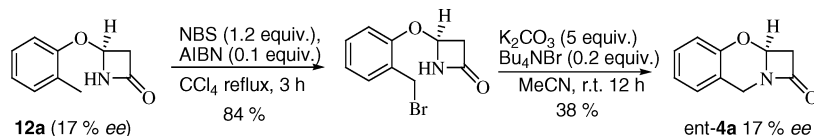
Scheme 5. Intramolecular N -benzylation leading to ent- 4a .
