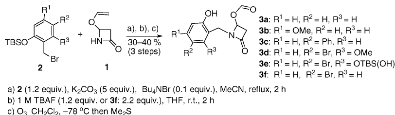
Scheme 3. Preparation of N -benzyl-substituted azetidinones 3 .
